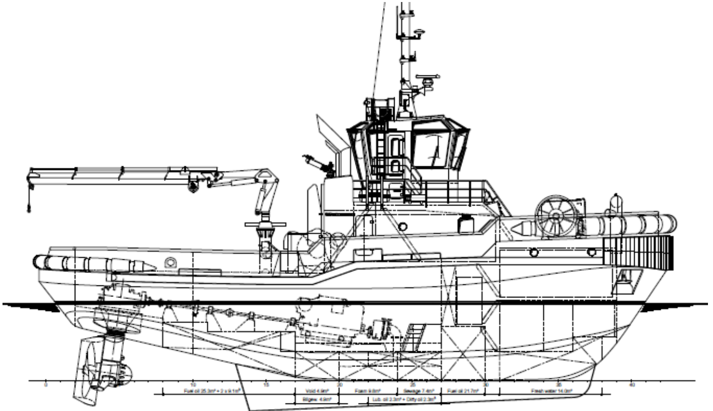
Main deck
