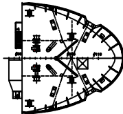
Forecastle deck.
